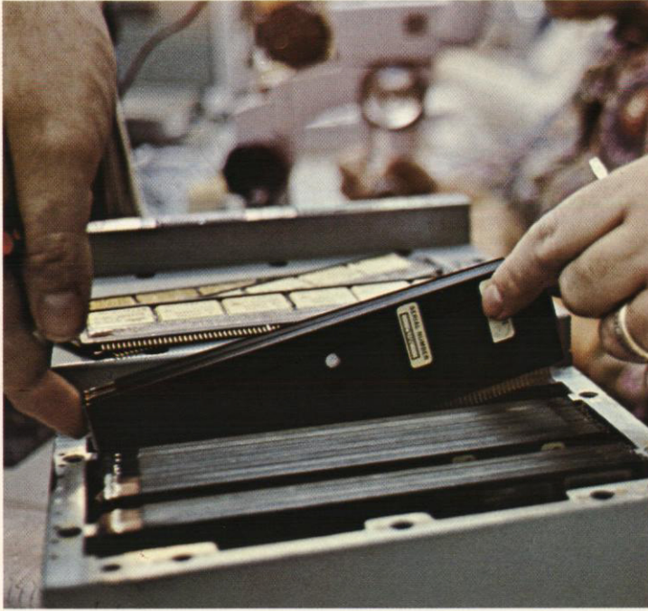
A logic module, containing twenty-four MEMAs mounted on submodule boards, is inserted into an airborne computer during assembly.
