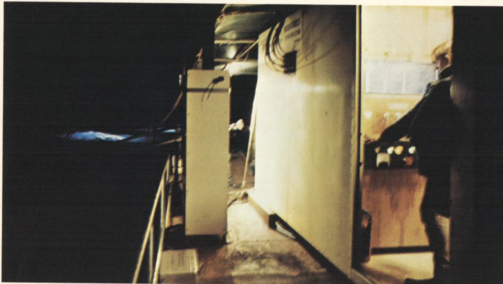
A bubble forms in the water behind the survey vessel from the discharge of the electrical energy stored in the high voltage capacitor bank at the ship's rail.
