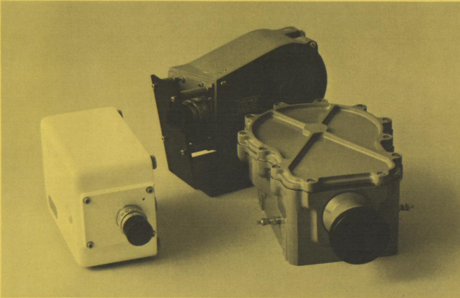
The DBM-8 camera, center, recorded John Glenn during his history-making Mercury flight. Model DBM-3, left, has been one of the workhorse cameras at Cape Kennedy for many years. This camera, mounted in a sealed capsule on board the Saturn first stage, records booster separation and is then ejected into the ocean and recovered. As many as 80 similar cameras are positioned at various locations on the launch pad to record the Saturn lift-off at close range. The DBM-10M1, right, was developed specifically for the Apollo program. It was used in initial unmanned flights of the Apollo capsule where it recorded flight instruments and the re-entry trail through the capsule window.
