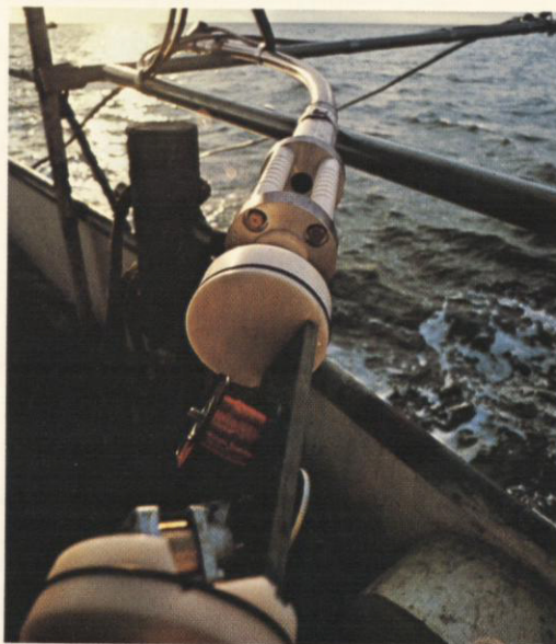
In the Wire Arc Seismic Section Profiler (WASSP), fine wire is automatically advanced every few seconds between high voltage insulators from a spool to the arcing electrodes, where it is explosively vaporized by up to 200,000 joules of electrical energy.
