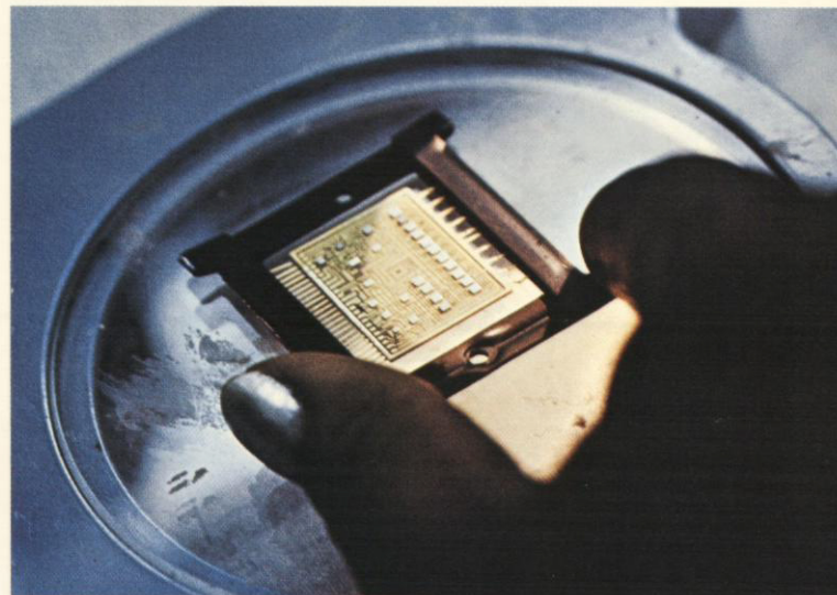
A MEMA with individual integrated circuit chips attached to the ceramic substrate is held in a handling fixture to prevent damage in the fabrication process prior to sealing.
