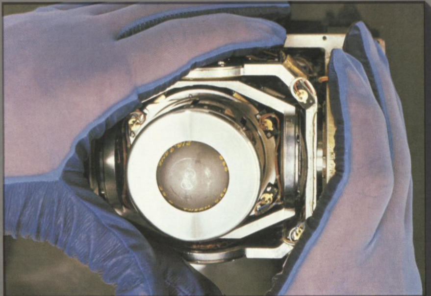
The smallest inertial navigator produced to date the FRSS platform is held in the gloved hands of an engineer in a dust free room. Sealed in its case, it will stand the rigors of aircraft environment and continuously provide the pilot with speed and position information.
