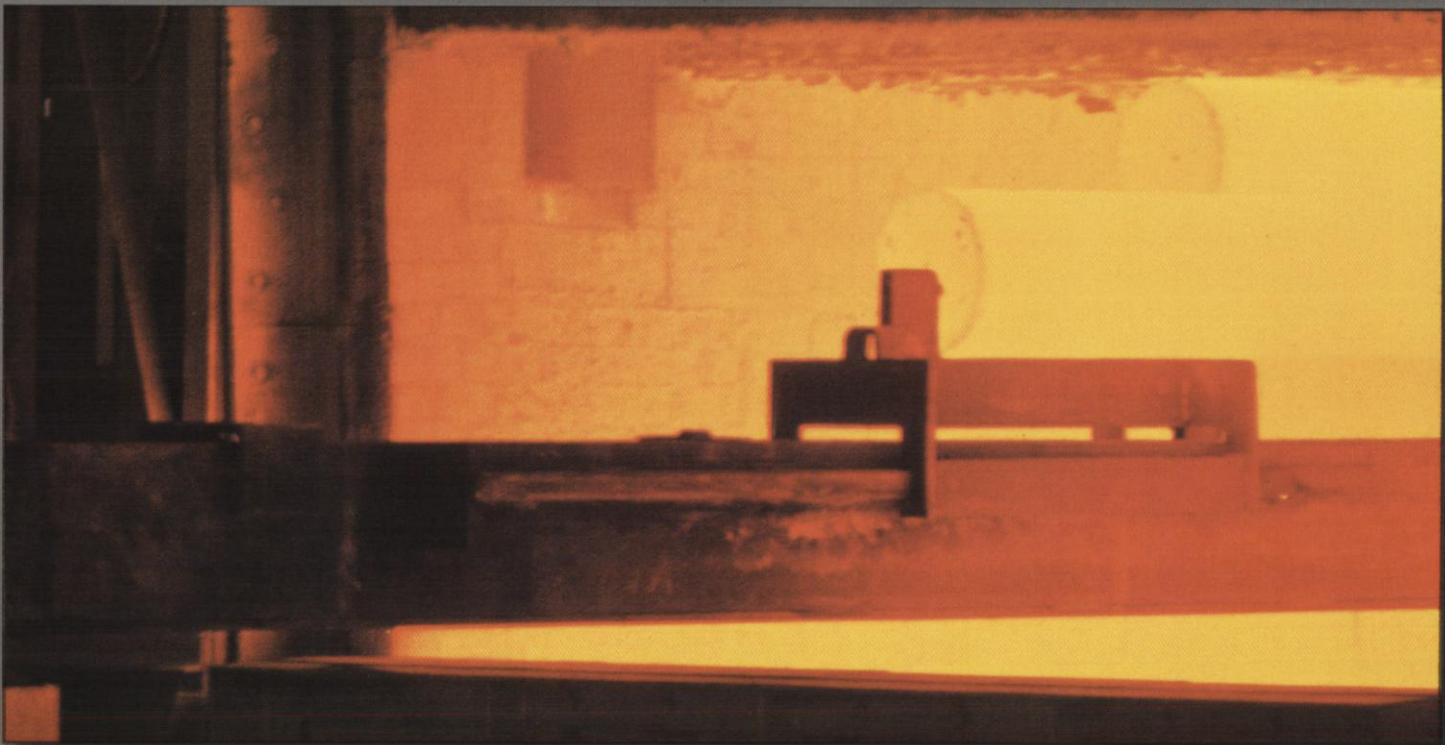
A 3,000-pound superalloy ingot produced by the double vacuum melting process is removed from a soaking furnace—later to be shaped and further treated for use in high strength, high temperature products.
