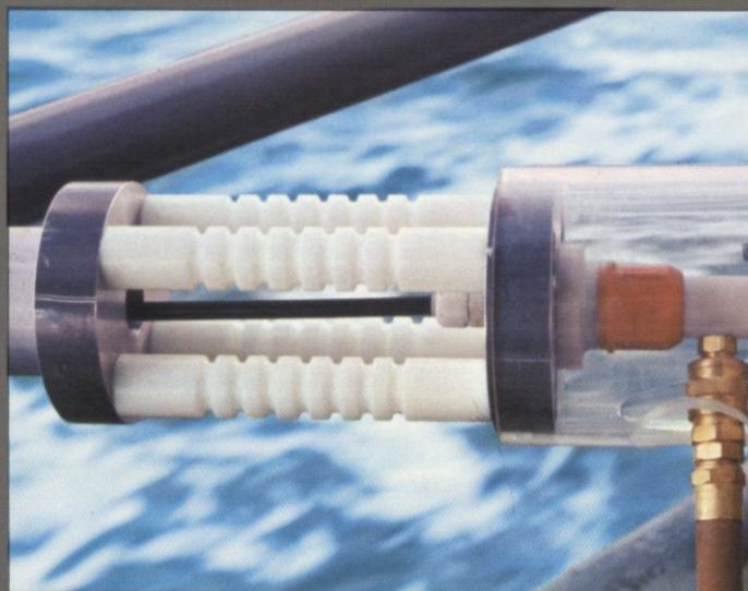
A hydraulically activated dispensing mechanism aboard ship (below) feeds wire to a Wire Arc Seismic Section Profiler (above). Towed behind the exploration vessel, the WASSP generates acoustic energy for mapping the ocean sub-bottom by exploding the wire with a high current electrical discharge.
